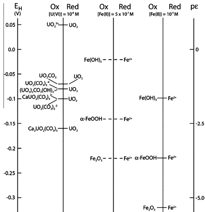
Fig. 2. Fe(III)/Fe(II) and U(VI)/U(IV) redox couples at pH 7, 3 \times 10^{-3} M bicarbonate, 1 \mu\text{M} U(VI), and 1 \text{ mM} \text{Ca}^{2+} . Reprinted with permission from Ginder-Vogel et al. (2006), copyright 2006 by the American Chemical Society.
