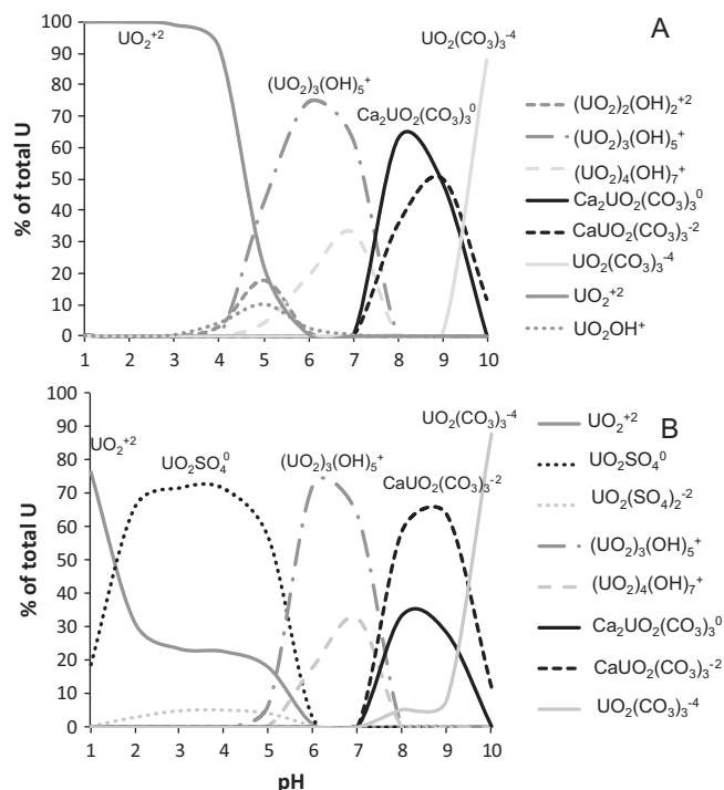
Fig. 1. Aqueous chemical speciation of U(VI) as a function of pH in simplified natural water matrix. Panel A was calculated with 0.1 mM U, 1 mM Ca, 10^{-3.5} atm \text{CO}_2 , and NaCl as an ionic strength buffer. In Panel B, 8 mM sulfate was added to the calculation. Calcite was allowed to precipitate in both simulations. Speciation was calculated with visual MINTEQ geochemical speciation code (Gustafsson, 2010) with uranyl equilibrium constants from (Guillamont et al., 2003; Dong and Brooks, 2006). Any species less than 1% of the total U was not plotted.
